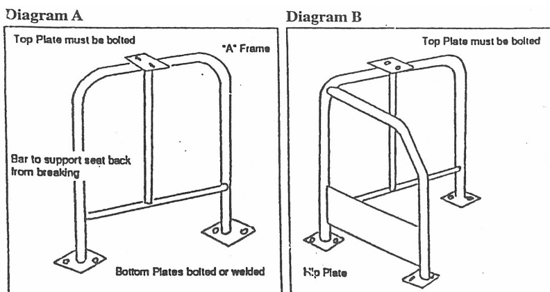
DIAGRAM .A. Mandatory safety frame design
